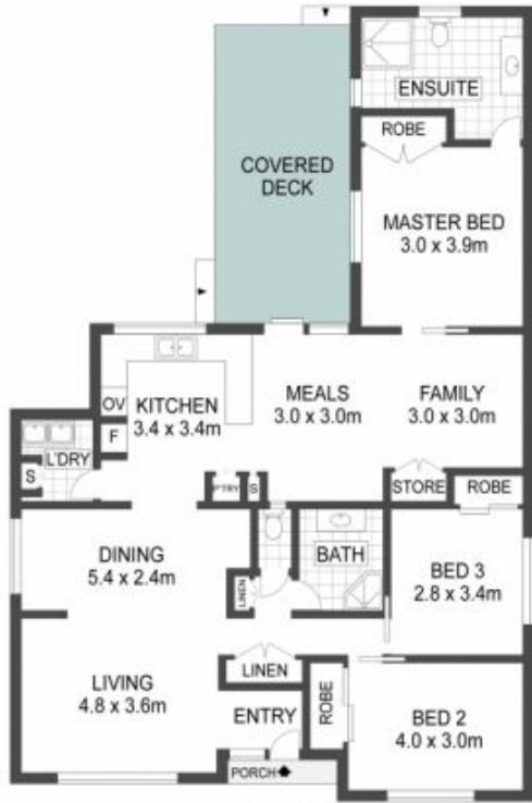
FLOOR PLAN
