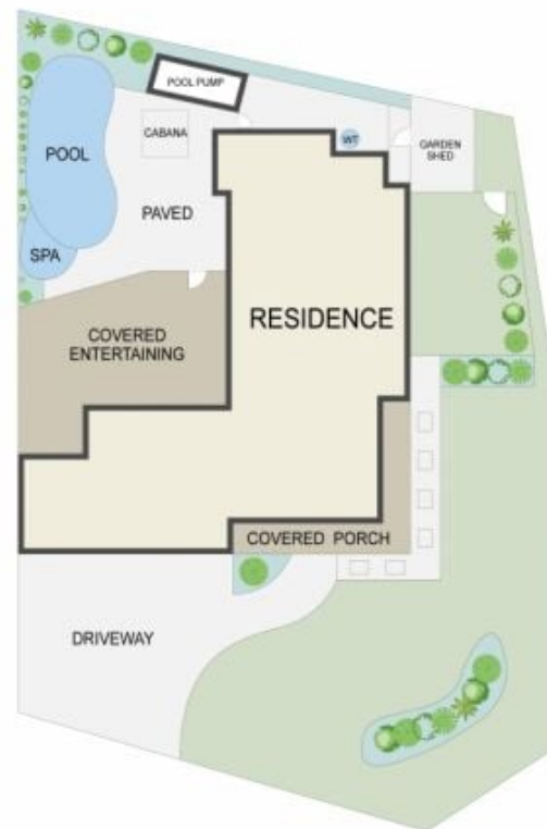
SITE PLAN
