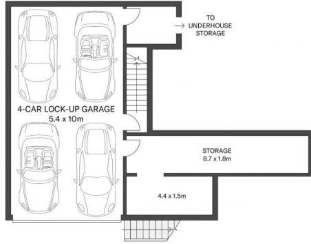
LOWER LEVEL
